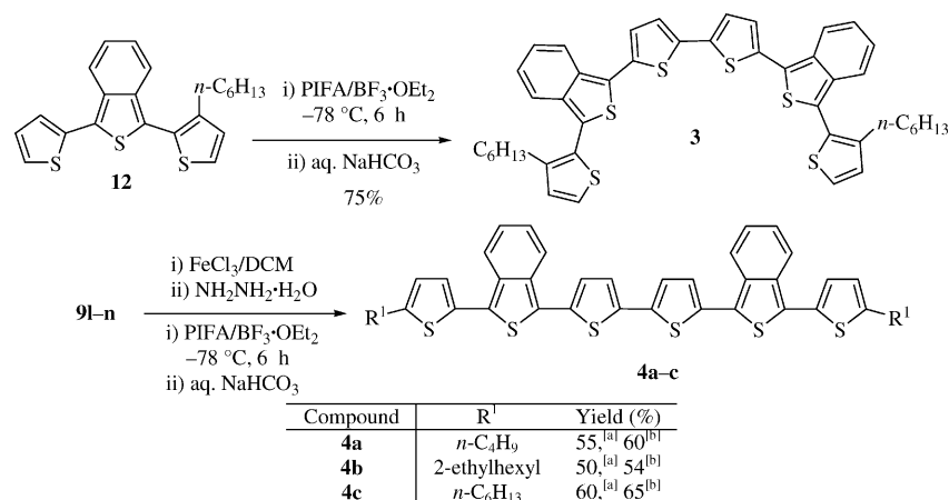
Scheme 9. [a] Yield obtained using FeCl 3 . [b] Yield obtained using PIFA/BF 3 ·Et 2 O.
