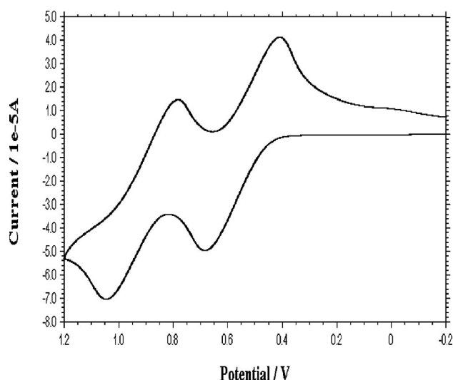
Figure 3. Cyclic voltammogram of 2d .
